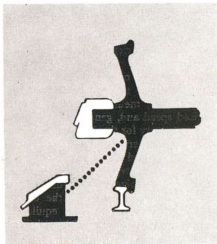
New "look" of GRS radiometer is at the hub of the wheel.
